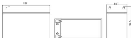
Faston flat connector 4,8 mm
