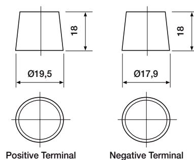
Positive Terminal
