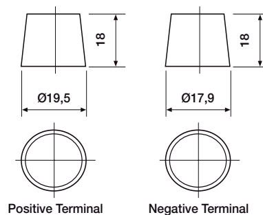
Positive Terminal
